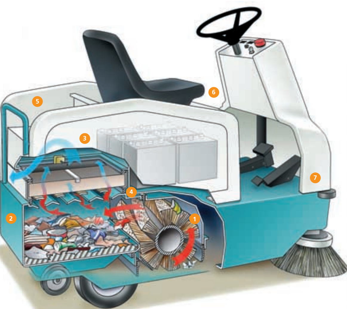
The Model 6100 offers the compact advantage when it comes to warehouse sweeping. It can maneuver down the most congested aisles and turn in the tightest spaces.
